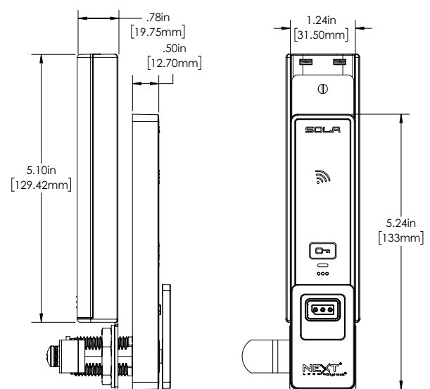
Digilock Sola 3 - Touch RFID Side View / Front View
