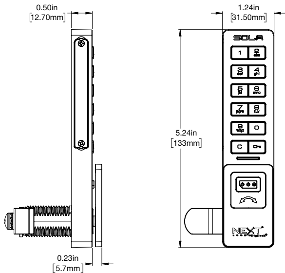
Digilock Sola 3 - Keypad Side View / Front View
