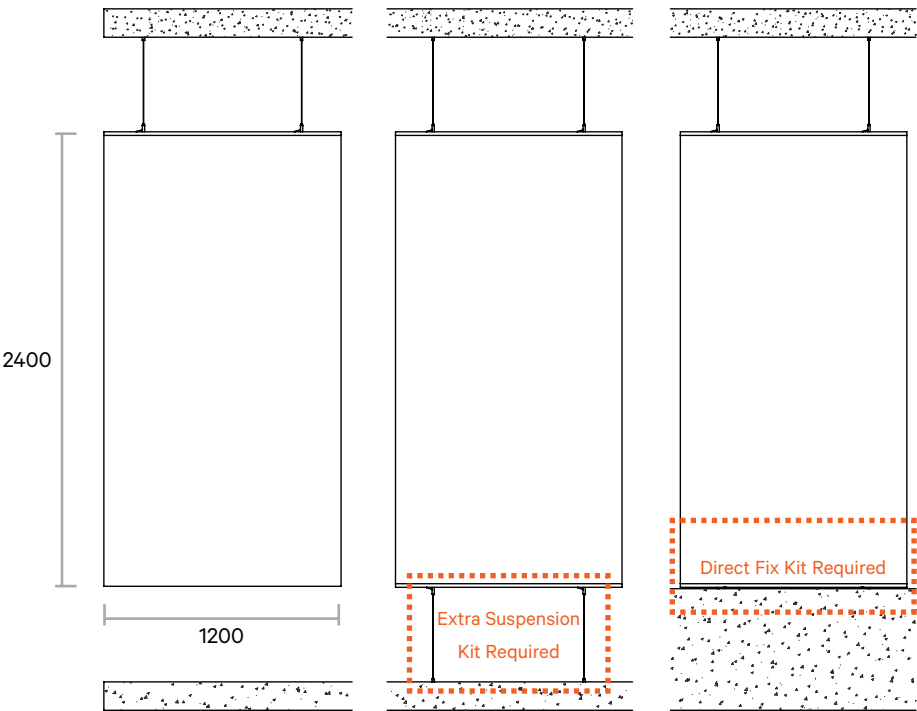
Suspended Top Free-hanging Base
