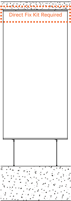
Direct Fixed Top* Suspended Base
