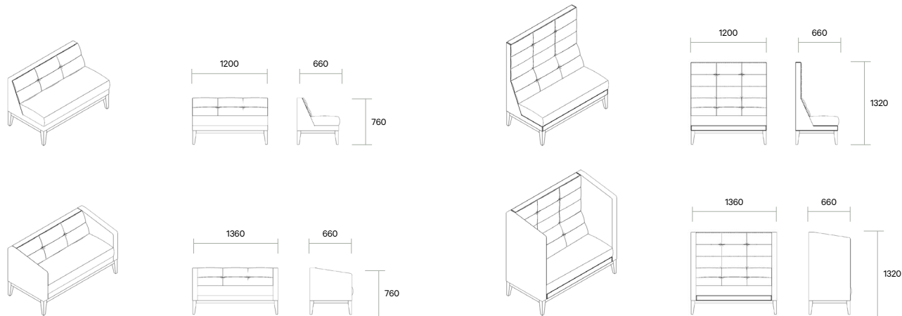
2 seater low back
