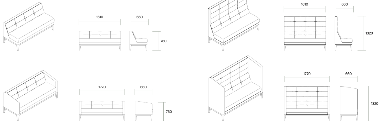
2.5 seater low back
