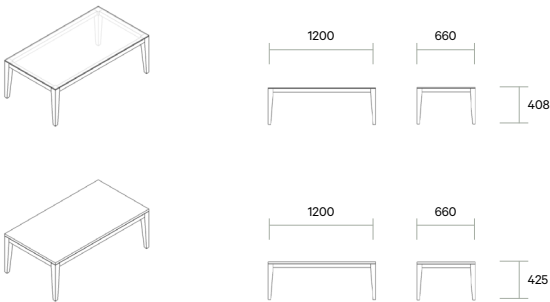
Rectangular coffee table - glass top + laminate top - 1200x660
