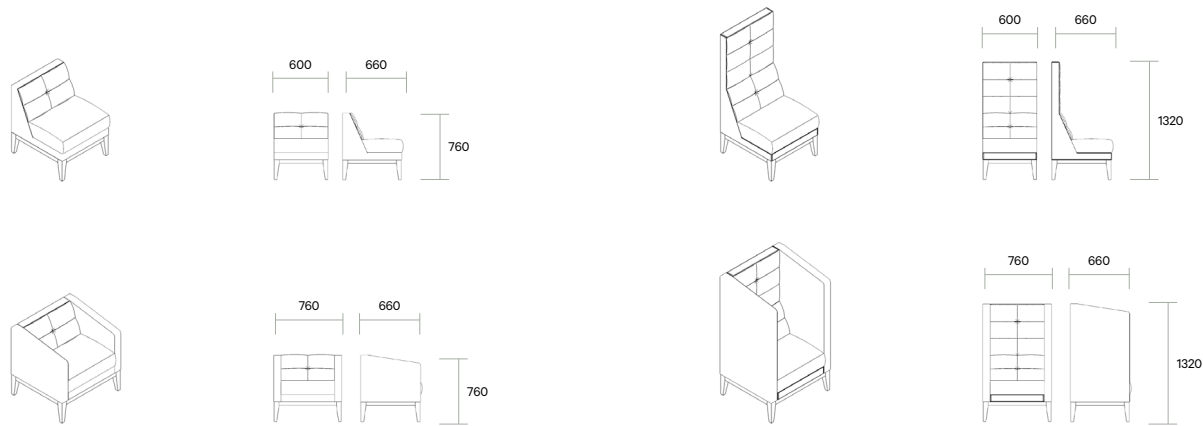
Chair low back
